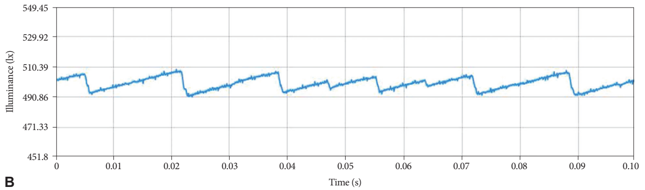
Supplementary Figure 1. Waveforms of the light-emitting diode light. The x-axis indicates time (sec) and the y-axis indicates illuminance (lx). (A) Control flicker light. Frequency, 120 Hz; mean illuminance, 501 lx (max, 709.2 lx; min, 286.8 lx); percent flicker, 40.27%; flicker index, 13.37%. (B) Reduced flicker light. Frequency, 120 Hz; mean illuminance, 499.7 lx (max, 508.8 lx; min, 491.1 lx); percent flicker, 1.78%; flicker index, 0.28%.
