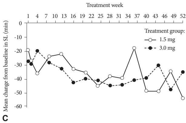
Supplementary Figure 1. Mean change from baseline for weekly TST (A), WASO (B), and SL (C) in the intent-to-treat population (observed case). SL: sleep latency, TST: total sleep time, WASO: wake time after sleep onset.
